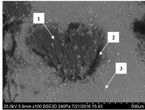
Fig. 6. SEM image of hemp concrete (500 \mu\text{m} ): (1) Hemp shiv (2) Porosity (3) Binder
