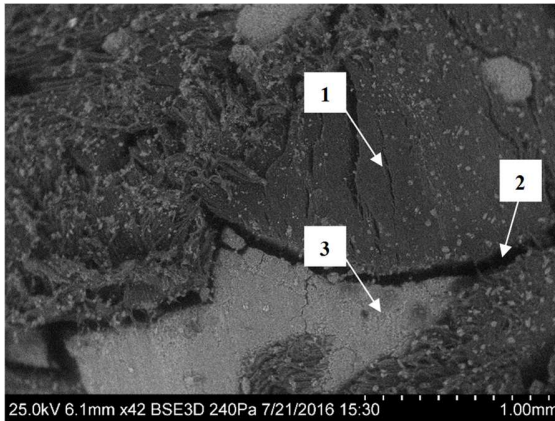
Fig. 5. SEM image of hemp concrete (1 mm): (1) Hemp shiv (2) Porosity (3) Binder
