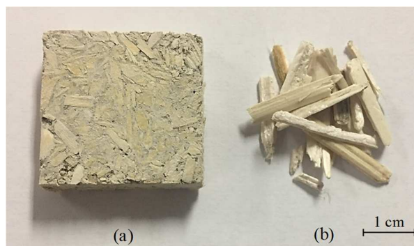
Fig. 1. Studied material (a) Hemp concrete (b) Hemp shiv
