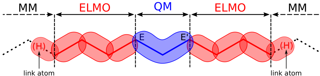
Figure 1. Schematic representation of the QM, ELMO and MM regions in the QM/ELMO/MM method. E and E' are the frontier atoms between the QM and ELMO subsystems.
