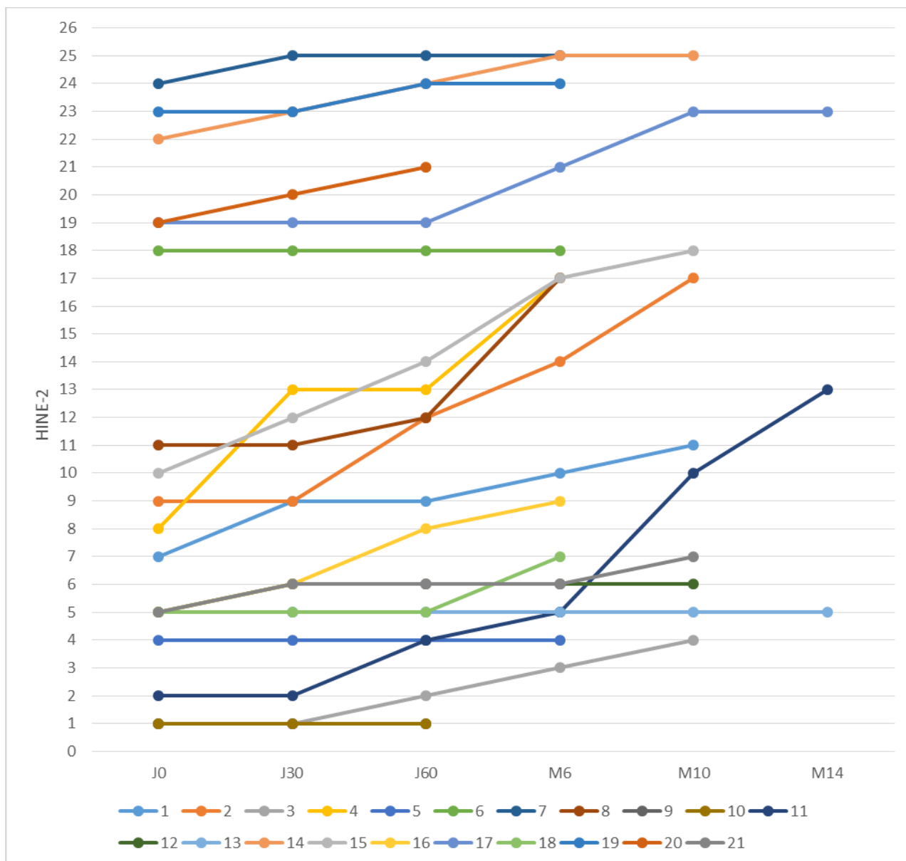
Figure 1: Evolution of HINE-2 score for each patient
