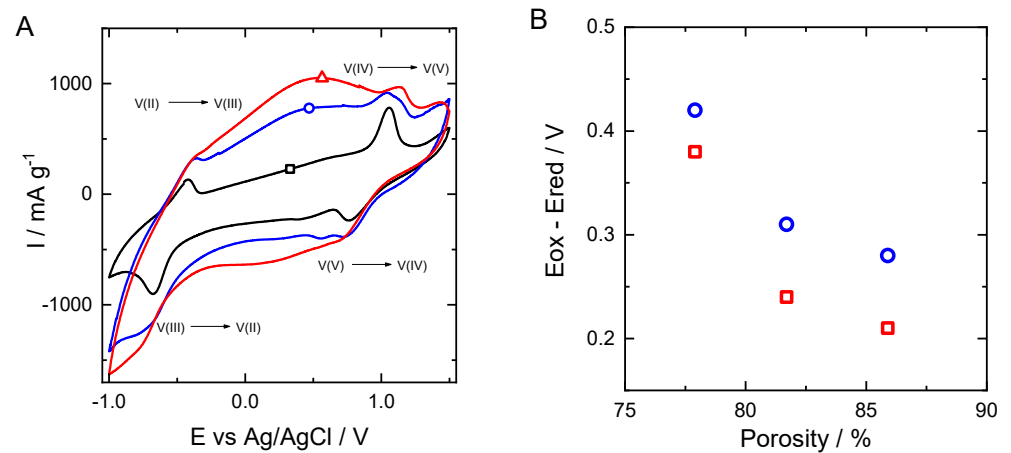
Figure 7. (A) Cyclic voltammograms recorded at 5 \text{ mV} \cdot \text{s}^{-1} in 0.15 \text{ M V(III)/V(IV)} solution prepared in 3 \text{ M H}_2\text{SO}_4 for samples SucNaCl0.80 ( \square ), SucNaCl1.00 ( \circ ) and SucNaCl1.25 ( \triangle ). (B) Differences between oxidation and reduction potential as a function of porosity: \text{V(V)/V(IV)} ( \circ ) and \text{V(III)/V(II)} ( \square ).
