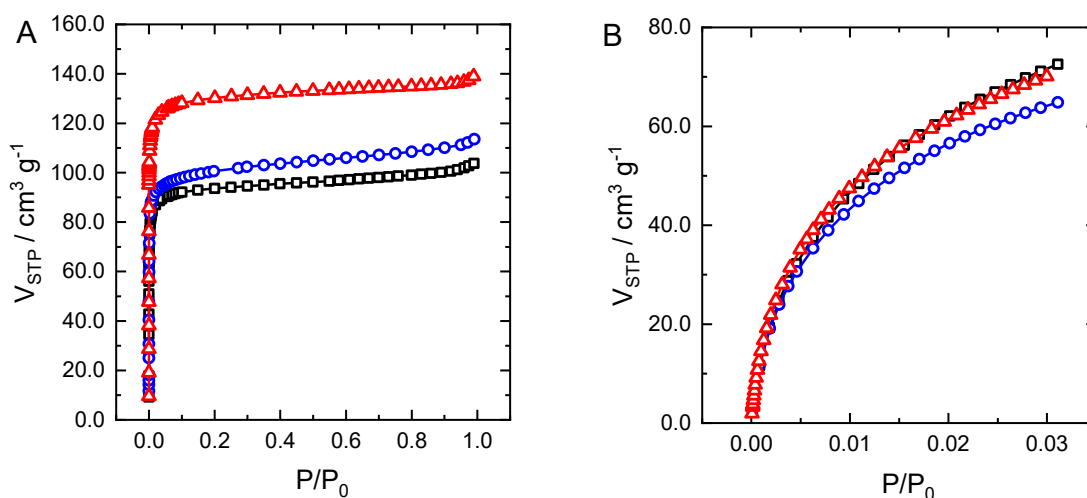
Figure 2. (A) Nitrogen adsorption isotherms at -196 \text{ }^\circ\text{C} , and (B) carbon dioxide adsorption isotherms at 0 \text{ }^\circ\text{C} for samples SucNaCl10.80 ( \square ), SucNaCl1.00 ( \circ ) and SucNaCl1.25 ( \triangle ).
