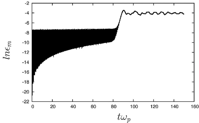
FIG. 8. Plot of the magnetic energy, on a logarithmic scale, as a function of time. The figure shows clearly the three different steps of the instability: the transient stage (characterized by high frequency oscillations due to the presence of high frequency modes), an exponential growth (of a low-frequency mode), and then the saturation phase. The simulation corresponds to case A (2D3V code).
