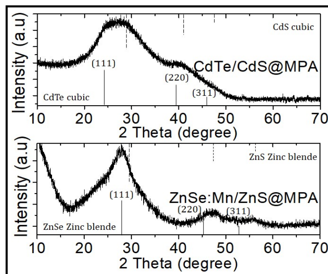
Figure 2: XRD pattern of ZnSe:Mn/ZnS@MPA and CdTe/CdS@MPA QDs.
