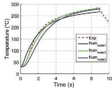
Fig. 9. Experimental temperature at the thermocouple versus numerical temperature evolution at nodes 1, 2 and 3 for h = 300kW/m^2/^{\circ}C .
