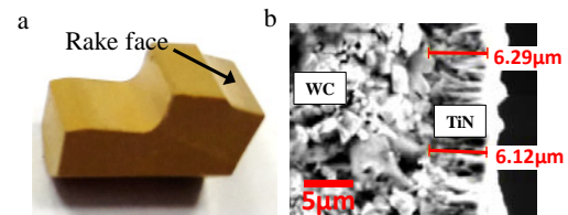
Fig. 3. (a) TiN-coated tool (made by EVATEC TOOLS); (b) Coating thickness.
