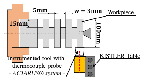
Fig. 4. Experimental setup.
