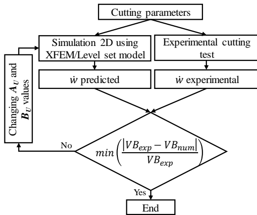
Fig. 2. Identification algorithm of the Usui wear parameters A_U and B_U .
