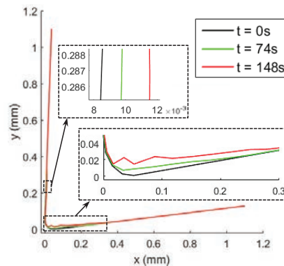
Fig. 11. Tool wear profile progress.
