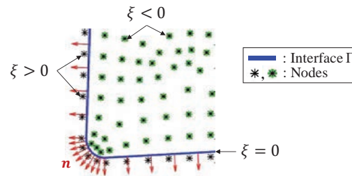
Fig. 6. Interface definition with a level set function for a coated structure.
