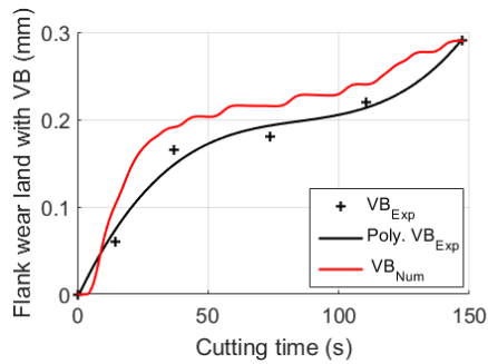
Fig. 12. Comparison between simulated and experimental wear for V_c = 150 m/min and f = 0.18 mm/rev.
