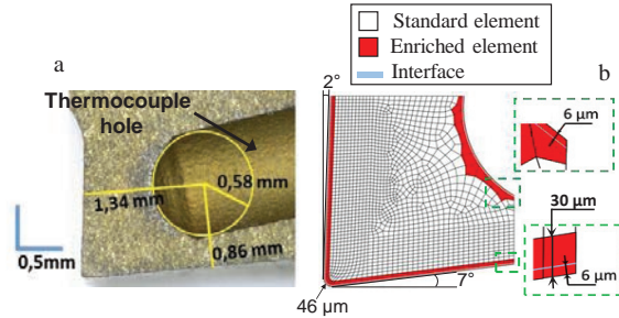
Fig. 5. (a) Cross section of the tool with the real dimensions of the thermocouple hole; (b) XFEM/Level-set mesh with the interface representation.
