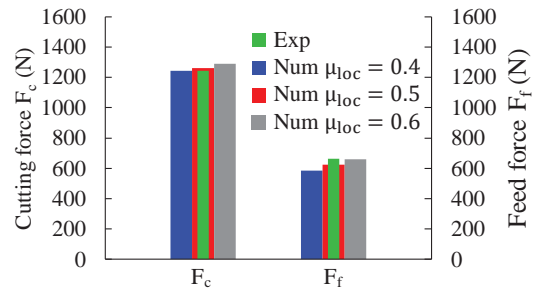
Fig. 8. Effect of the local friction coefficient on the forces.
