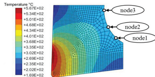
Fig. 10. Distribution of the temperature at t = 9s .
