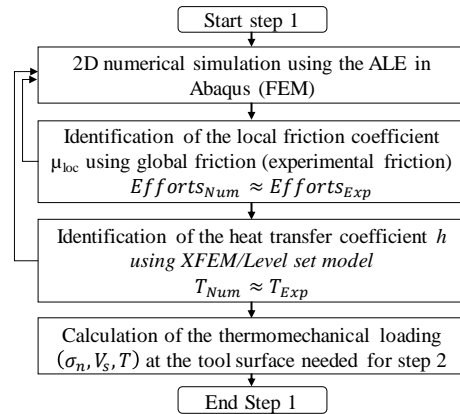
Fig. 1. Sequential step 1 of the proposed approach to identify the ALE model parameters and to calculate the thermomechanical loading required for step 2.
