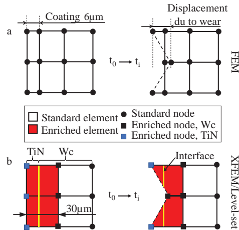
Fig. 7. Nodal displacement du to wear for: (a) FEM; (b) XFEM/Level set model.
