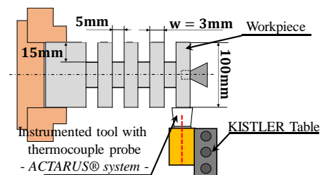
Fig. 4. Experimental setup.
