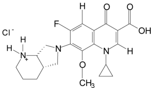
Scheme 1. Chemical structure of MOXI.
