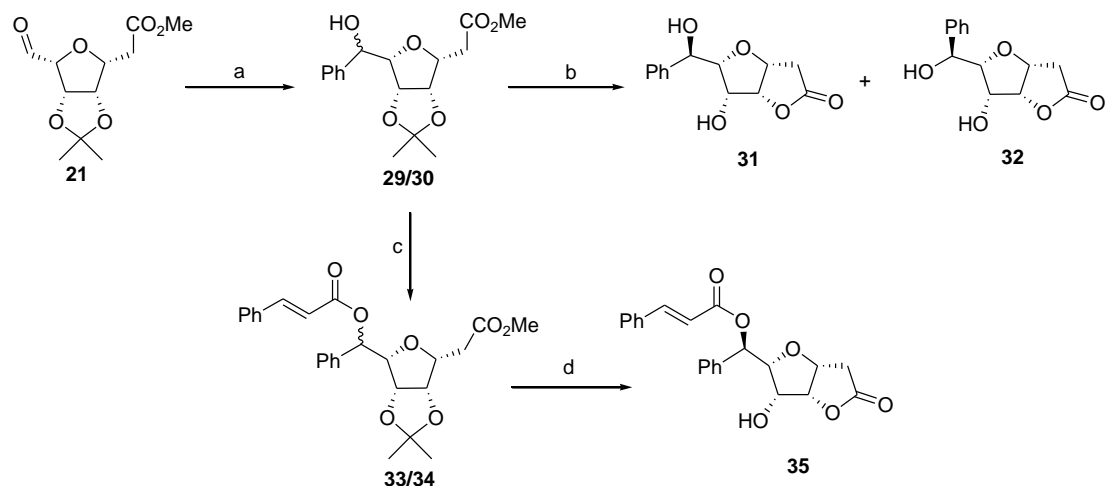
Scheme 4. Reagents and conditions: a) PhMgBr, Et 2 O, 0 °C, ratio 29/30 : 65/35; global yield 35 %; b) TFA/H 2 O (1/1 v/v), 31 : 25 % and 32 : 15 %. c) cinnamoyl carboxylic acid, DCC, DMAP, CH 2 Cl 2 , 53 %, ratio 33/34 : 65/35; d) TFA/CH 2 Cl 2 (1/1 v/v), 56 %.
