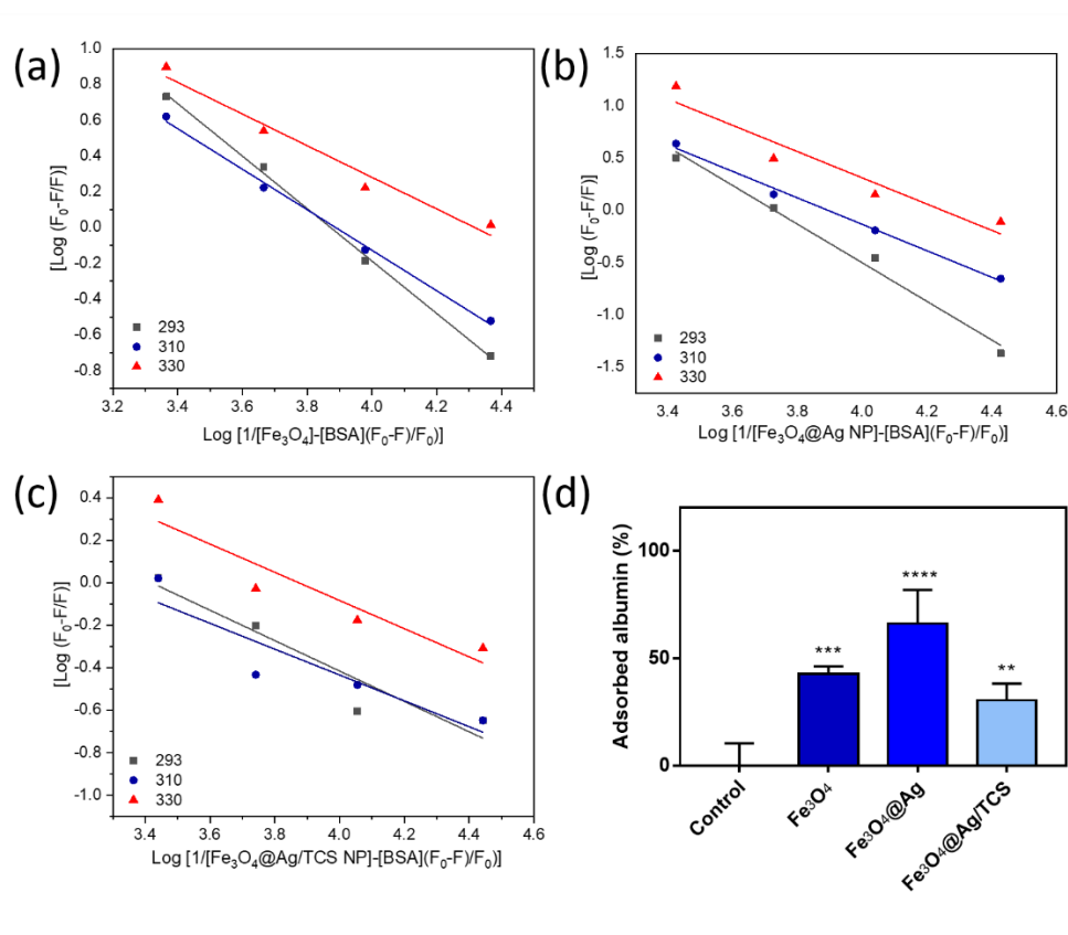
Figure 5. Plot of \text{Log}((F_0-F)/F) vs. \text{Log}(1/([\text{NP}]-[\text{BSA}])(F_0-F)/F_0)) for (a) \text{Fe}_3\text{O}_4 NPs and (b) \text{Fe}_3\text{O}_4\text{@Ag} NPs, and (c) \text{Fe}_3\text{O}_4\text{@Ag/TCS} NPs incubated with albumin, as a function of the temperature; (d) adsorbed albumin (%) after the incubation of 0.4 \text{ g.L}^{-1} of protein with 200 \mu\text{g mL}^{-1} of \text{Fe}_3\text{O}_4 NPs, \text{Fe}_3\text{O}_4\text{@Ag} NPs, and \text{Fe}_3\text{O}_4\text{@Ag/TCS} NPs. ** p < 0.0013 , *** p < 0.0006 , and **** p < 0.0001 , comparing to control, using Tukey’s multiple comparisons test.
