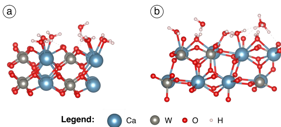
Figure 8. Adsorption of eight water molecules, which corresponded to a monolayer, onto (001) (a) and (112) (b) scheelite surfaces. The dashed lines represent hydrogen bonds.
