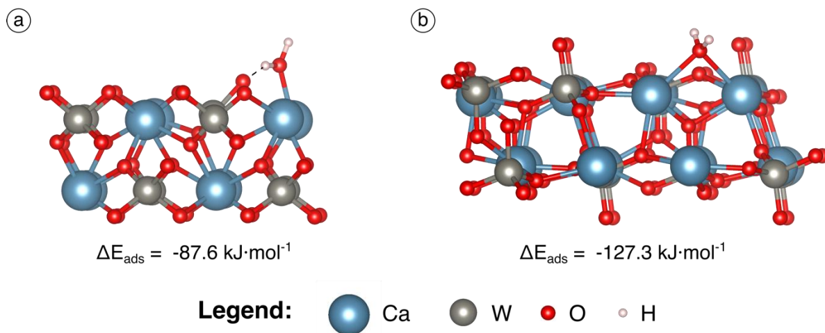
Figure 5. Adsorption of dissociated water molecule with short OH-H distance onto (001) (a) and (112) (b) scheelite surfaces. Only the upper part of the surfaces is displayed here. The dashed lines represent hydrogen bonds.
