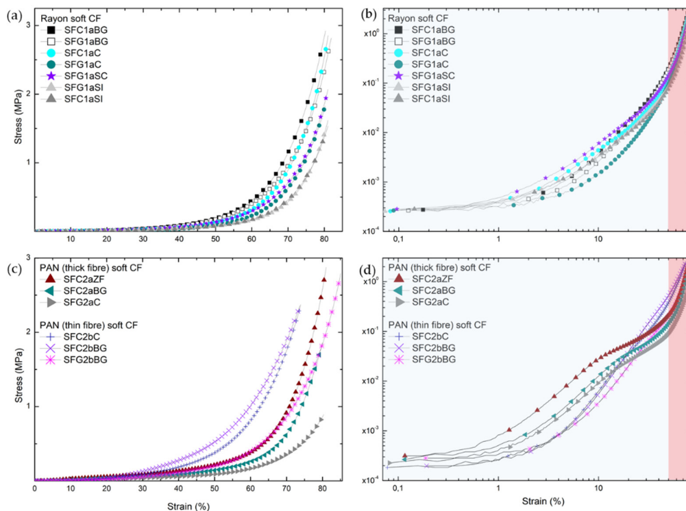
Figure 2. Stress-strain characteristics of soft carbon felts (CFs), subjected to uniaxial compression along their out-of plane (OP) ( z ) direction, derived from: (a) Rayon-derived and (c) polyacrylonitrile (PAN)-derived (thin and thick fibers); Logarithmic representations of (a) and (c) are given in (b) and (d), respectively, with indication of the compression zones influenced by different deformation regimes (“non-linear elastic”—transparent blue and “solid”—transparent red zone).
