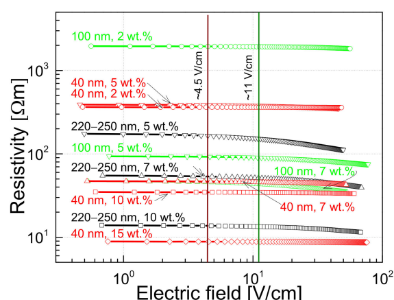
Figure 3. Dependences of the sample resistivity on the applied electric field at 290 K.
