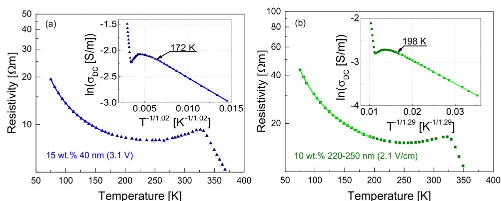
Figure 4. Changes of sample resistivity as a function of temperature for composites filled with 15 wt.% of OLC particles of size 40 nm (a), and with 10 wt.% of OLC particles of size 220–250 nm (b). Dots represent experimental results and solid lines represent fits for tunneling (Equation (3)). Insets represent fitting for variable-range hopping (Equation (4)). The indicated electrical field values are the values applied to the sample at room temperature (290 K).
