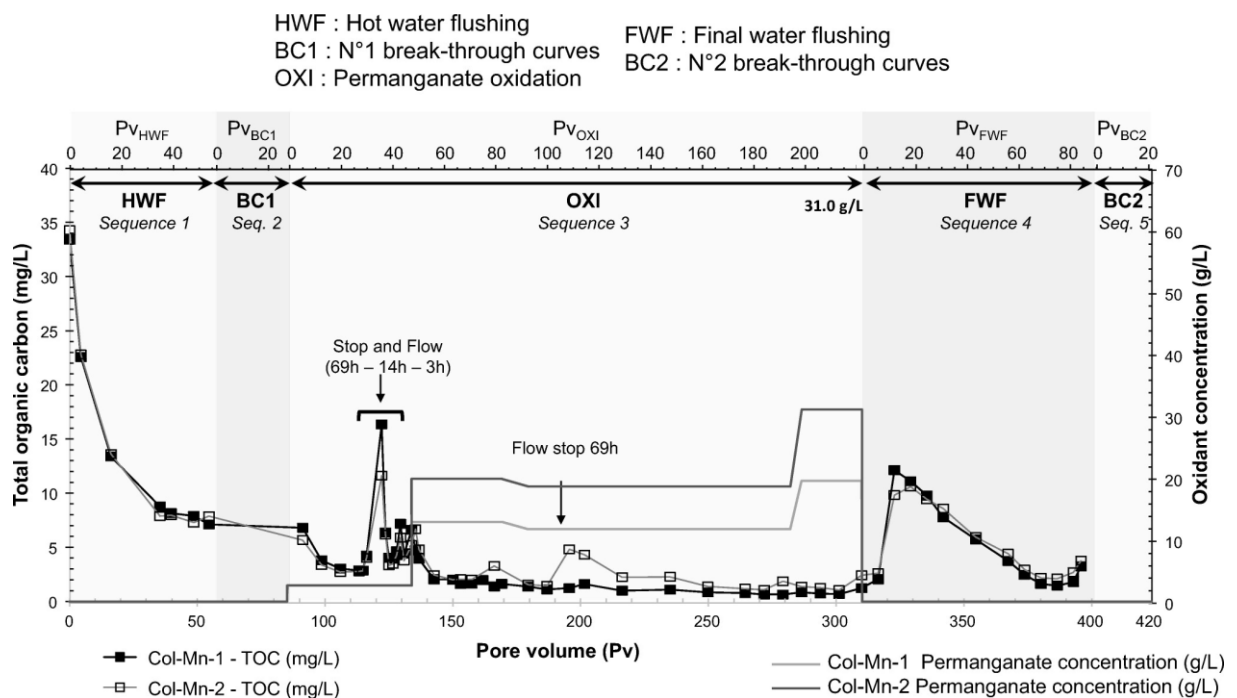
Fig. 4: Total organic carbon (TOC) values in the outgoing leachates from Col-Mn-1 and Col-Mn-2 from sequence 1 to 5 (hot water flushing (HWF), n°1 break-through curves (BC1), oxidation (OXY), final water flushing (FWF), and n°2 break-through curves (BC2)), overlapped with the oxidant concentrations applied in Col-Mn-1 and Col-Mn-2. The volumes eluted from the columns are given as total pore volumes (bottom X-axis) and as the pore volume (Pv) of each step (top X-axis)
