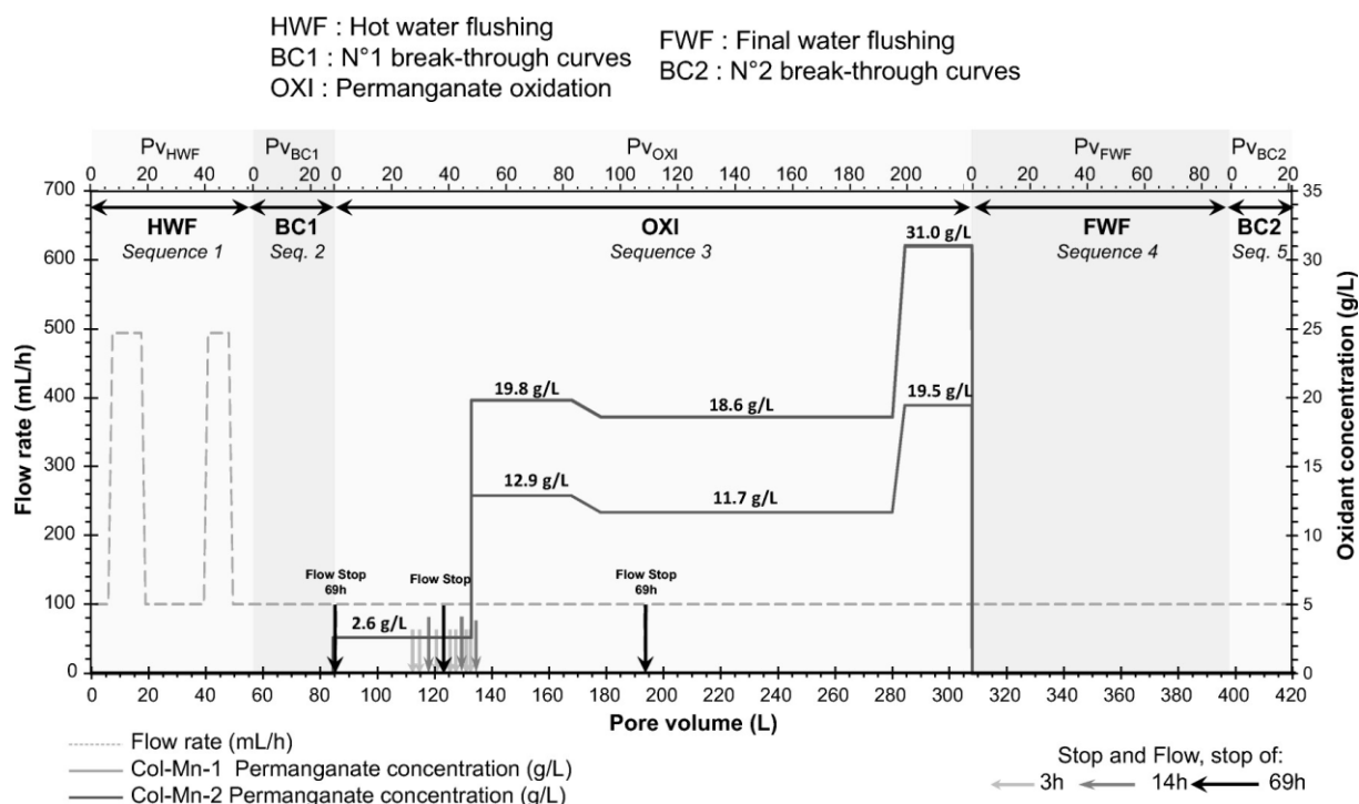
Fig.1: Injection protocol for permanganate-treated columns — 5 steps: hot water flushing (HWF); n°1 break-through curves (BC1); oxidation (OXI); final water flushing (FWF); and n°2 break-through curves (BC2). The volumes eluted from the columns are given as total pore volumes (bottom X-axis) and as the pore volume (Pv) of each step (top X-axis)
