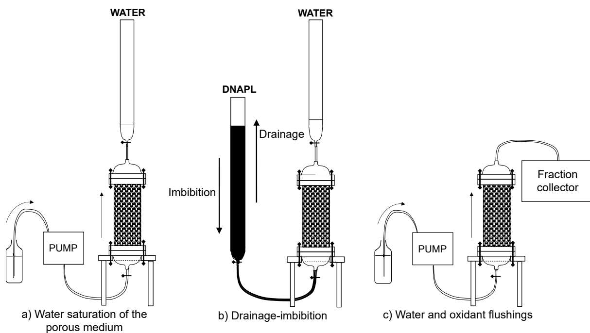
Figure S1: Diagram of a) water saturation of the porous medium; b) drainage – imbibition; and c) water and oxidation flushing steps.
