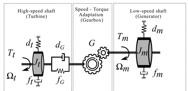
Fig. 4 Two mass schematic model of WPS drive train
