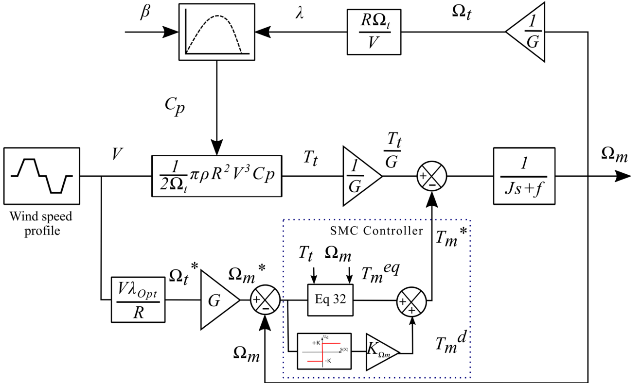
Fig. 17 TSR based MPPT algorithm using SMC controller
