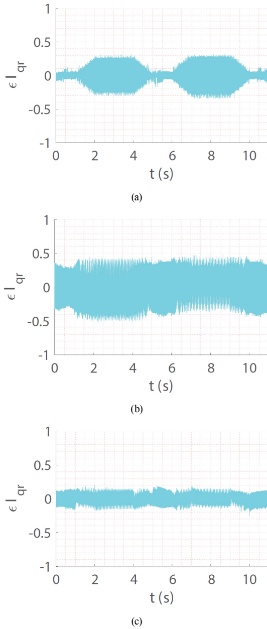
Fig. 30 DFIG Current tracking error ( I_{qr} tracking error); (a) PI; (b) SMC; (c) ST
