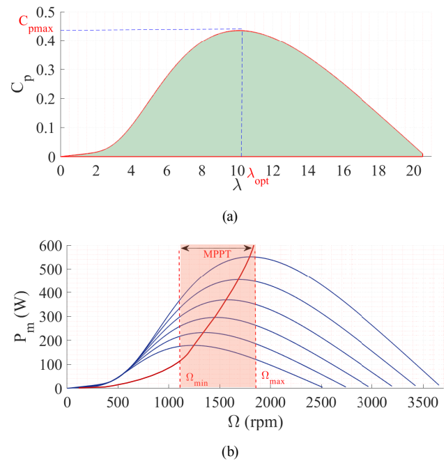
Fig. 7 Principle of the MPPT operation (a) maximum power coefficient (b) available aerodynamic power
