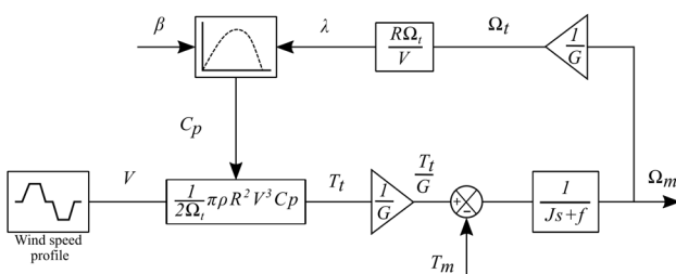
Fig. 5 The overall model of a variable-speed WPS
