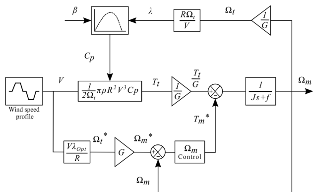
Fig. 8 Principle of the TSR based MPPT algorithm
