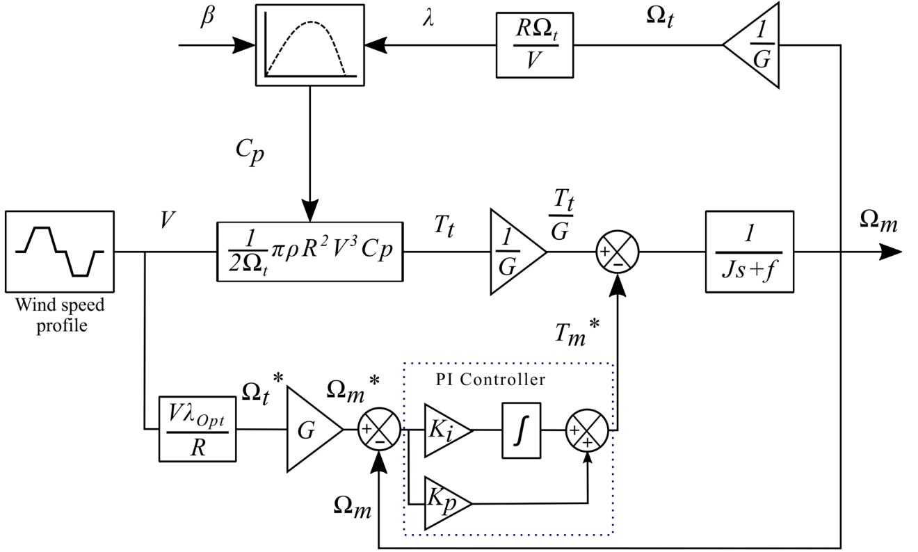
Fig. 16 TSR based MPPT using PI controller
