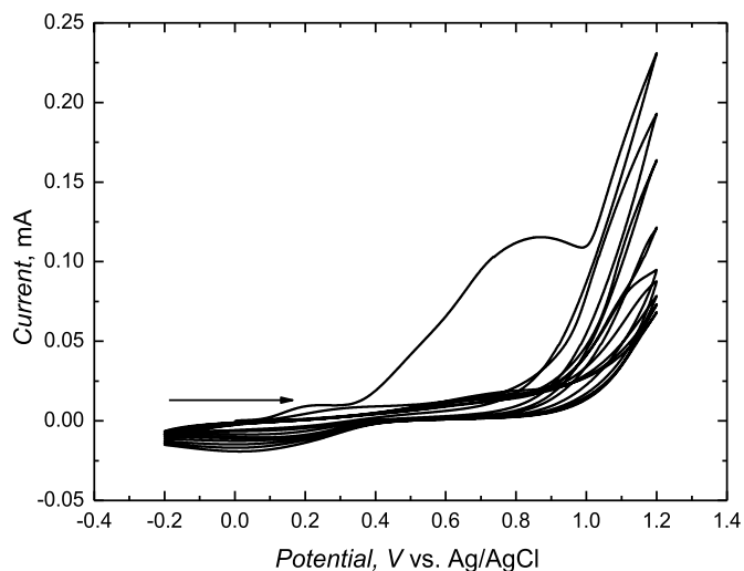
Fig. 1. The multi-cyclic potentiodynamic curve for the glassy carbon working electrode ( 0.38 \text{ cm}^2 ) in the 5 mL 0.01 M KCl solution of 2.5 mM 2-APBA, 10 mM ANI, and 200 \mu\text{L} of E2152 suspension ( 5 \times 10^9 \text{ cells mL}^{-1} ) at a scan rate of 25 \text{ mV s}^{-1} . Currents decrease in consecutive cycles.
