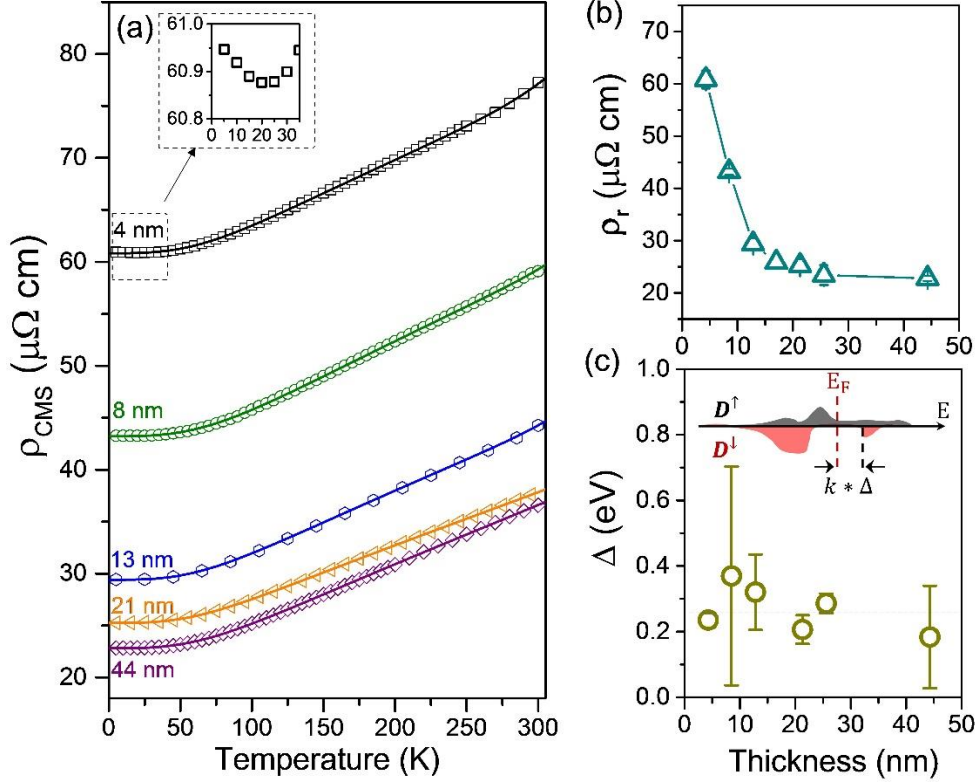
Fig. 3. Evolution of CMS resistivity with temperature. (a) Resistivity versus temperature for the \text{Co}_2\text{MnSi} thickness series. Solid lines are the fits to experimental data with eq. (5). In the inset, a zoom of the \rho_{CMS}(T) curve in the low-temperature range for the 4 nm \text{Co}_2\text{MnSi} film is shown. (b) \text{Co}_2\text{MnSi} residual resistivity versus thickness. (c) Distance between the Fermi energy and the bottom of the minority spin conduction band, \Delta , obtained from the fit of \rho_{CMS} vs. T with eq. (5) for the entire thickness series. A schematic of the DOS for both spins is shown as an inset.
