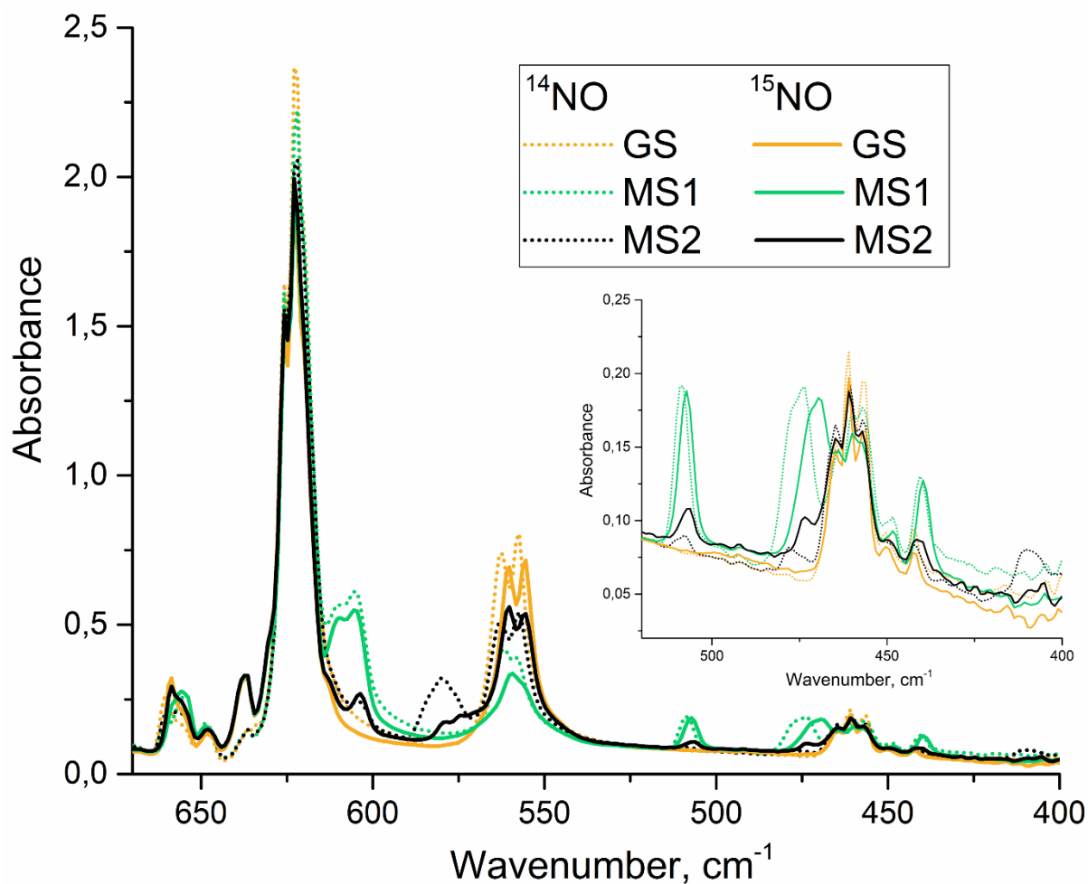
Fig. 6. The range of 670-400 \text{cm}^{-1} of IR-spectra of \text{trans-}[\text{Ru}^{15}\text{NO}(\text{py})_4\text{F}](\text{ClO}_4)_2 in GS, MS1 and MS2 (solid lines) and corresponding data of \text{trans-}[\text{Ru}^{14}\text{NO}(\text{py})_4\text{F}](\text{ClO}_4)_2 (dotted lines), KBr pellet. Insert shows the range 520-400 \text{cm}^{-1} .
