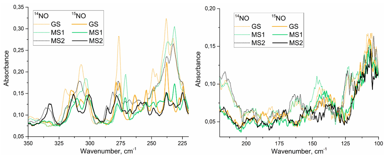
Fig. 7. The ranges of 350-200 (on the left) and 220-100 (on the right) \text{cm}^{-1} of IR-spectra of \text{trans-}[\text{Ru}^{15}\text{NO}(\text{py})_4\text{F}](\text{ClO}_4)_2 in GS, MS1 and MS2 (solid lines) and corresponding data of \text{trans-}[\text{Ru}^{14}\text{NO}(\text{py})_4\text{F}](\text{ClO}_4)_2 (dotted lines), PE pellet.
