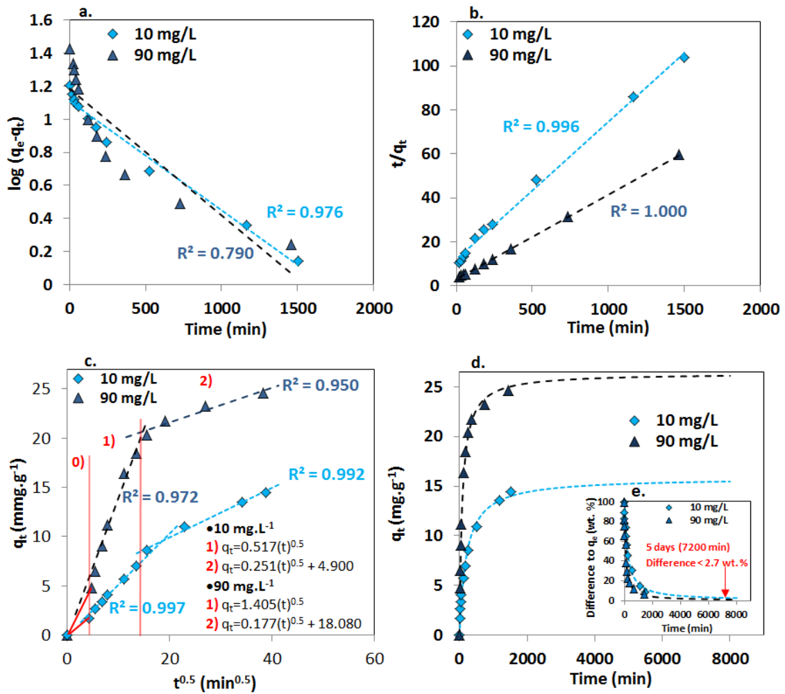
632 Figure 9. Adsorption kinetics of MB on X_12.5 carbon xerogel: (a) pseudo-first order plot, 633 (b) pseudo-second order plot, (c) intra-particle diffusion plot, and (d) fit of the pseudo- 634 second order to the adsorbed amount as a function of time for initial MB concentrations of 10 635 and 90 mg L -1 at 25°C; the inset (e) shows the difference between the two curves.
