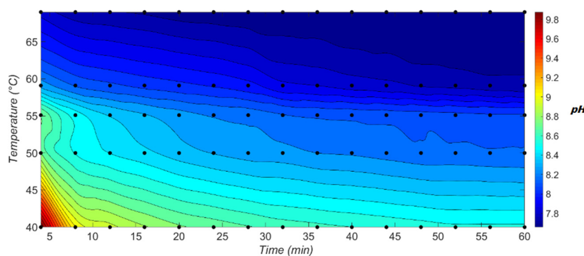
Figure 4. pH evolution over time at different temperatures [29]. Figure credit: N. Djoudi, M. Le Page Mostefa, and H. Muhr: Influence of Temperature on Cobalt Hydroxide Precipitation for Recovery from Battery Leachates. Chem. Eng. Technol. 2021. vol. 44, no. 6, pp. 962–971. Copyright Wiley-VCH GmbH.
