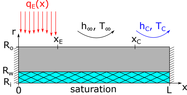
Figure 3: Model of the cylindrical heat pipe with one heat flux source and one temperature source
