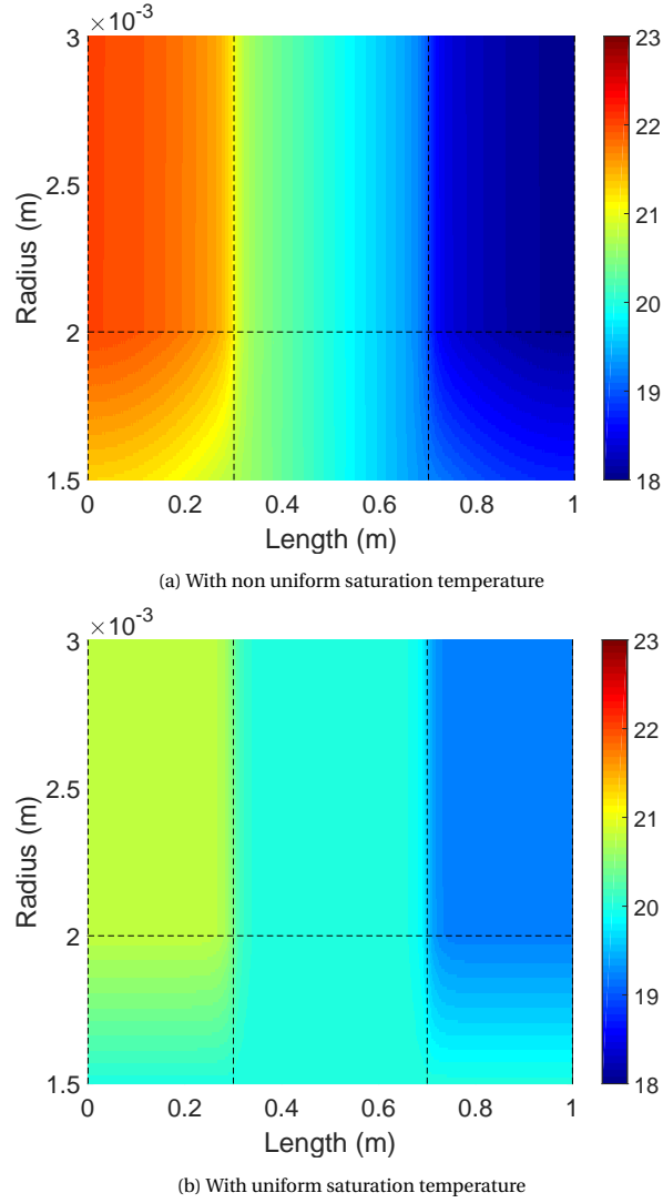
Figure 11: Temperature fields (°C) for micro heat pipe with an operating temperature of 20°C
