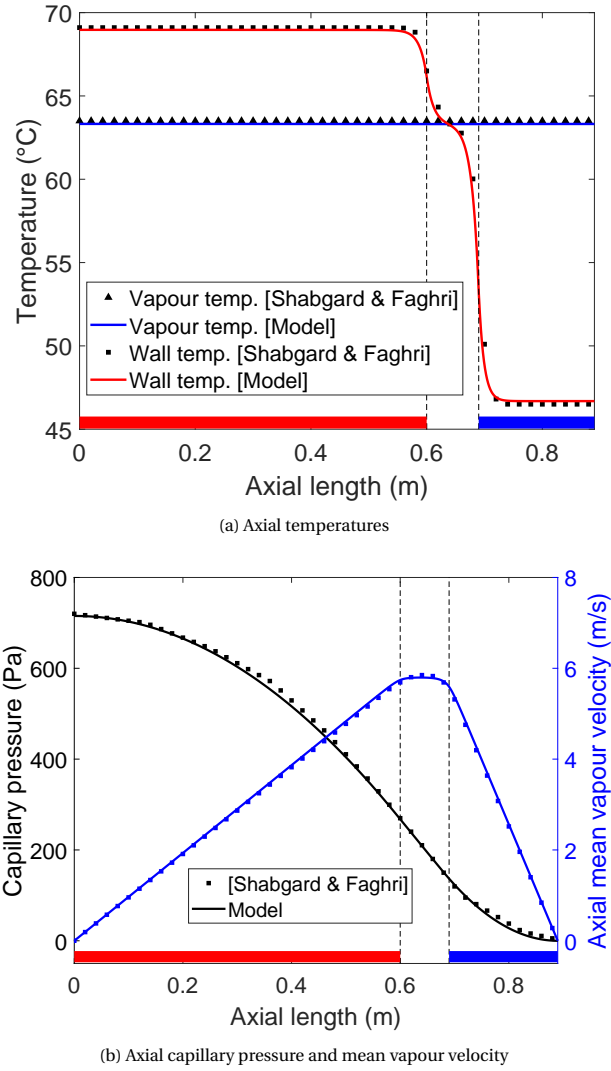
Figure 4: Case A - Comparison with results from Shabgard and Faghri [7]
