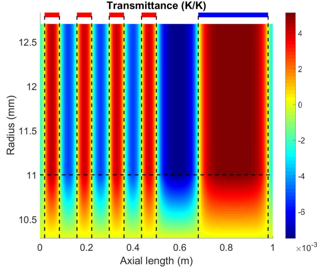
Figure 9: Case B with additional heat losses ( h_{\infty} = 10 \text{ W.m}^{-2}.\text{K}^{-1} ) - Thermal transmittance field ( W_{sat} from Eq. (48)) of \theta from the temperature difference \bar{T}_{sat} - T_{\infty}
