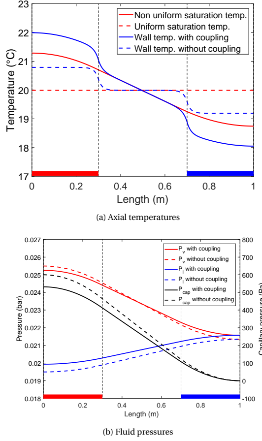
Figure 10: Micro heat pipe with an operating temperature of 20°C
