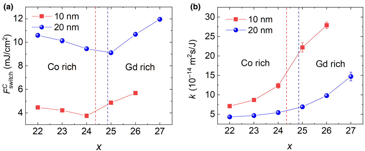
FIG. 3. Quantitative description of the key features of AO HIS Gd_x(FeCo)_{100-x} state diagrams. (a) The critical switching fluence F_{switch}^C obtained from the intercept of linear fit of F_{switch} on the x axis is plotted as a function of Gd concentration. (b) Evolution of the slope k extracted from the linear fit of F_{switch} as a function of Gd concentration.
