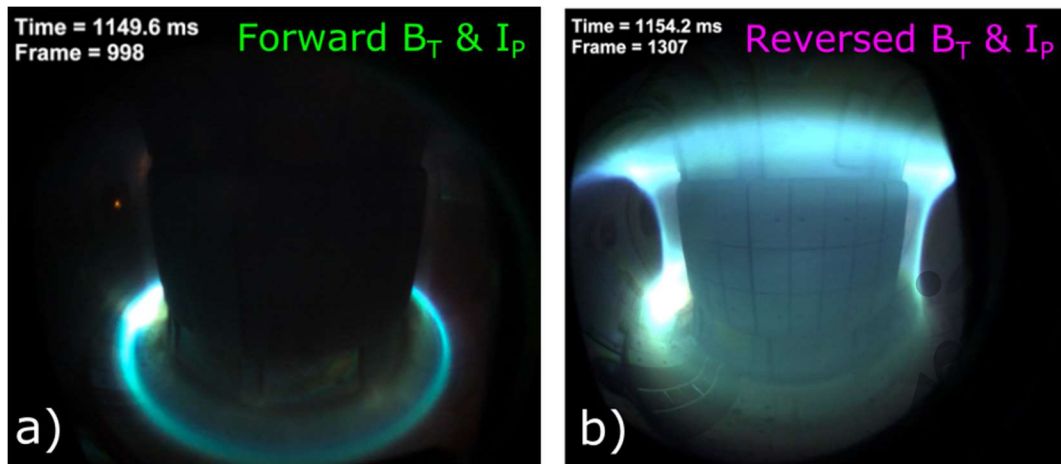
Fig. 8: Fast camera image of nitrogen radiation in experiments with forward (A) and reversed (B) direction of toroidal magnetic field and plasma current. In the forward field, the seeded nitrogen creates a radiation manile in the vicinity of the X-point, while in the reversed field, the seeded gas spreads along the HFS to the top of the vacuum vessel. In the latter case, a stable detached discharge cannot be achieved.
