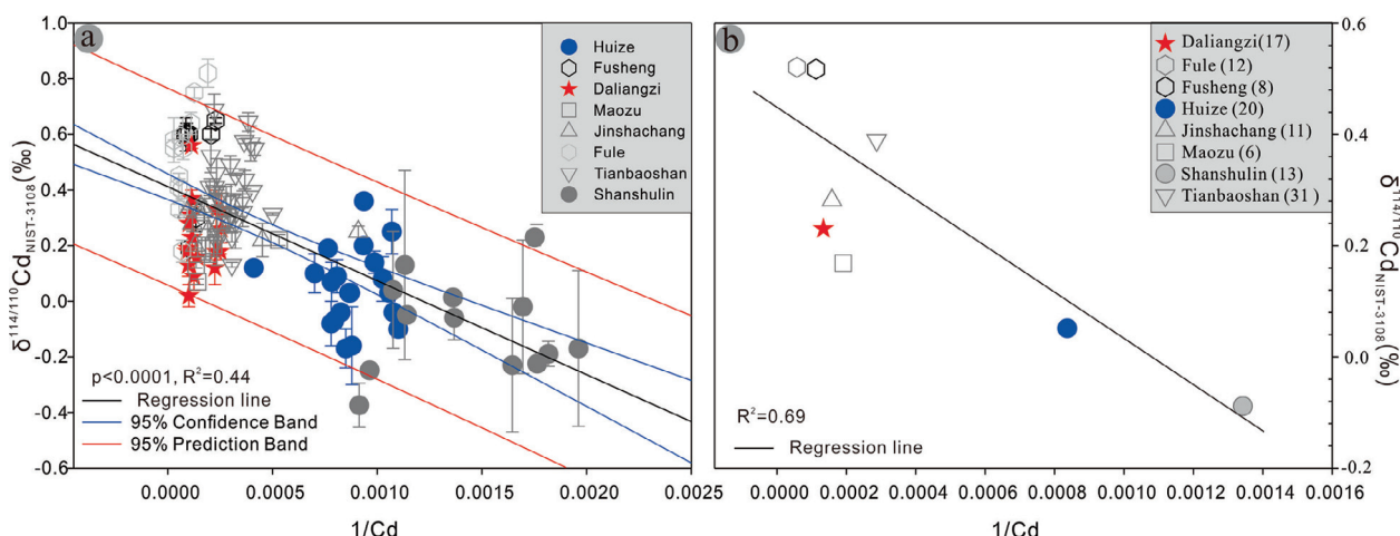
Fig. 7. Plot of average 1/Cd vs. average \delta^{114/110}\text{Cd} values of sphalerite from eight Zn–Pb deposits in the SYG area. For data sources see Fig. 6 and Supplementary Data (Table S4).
