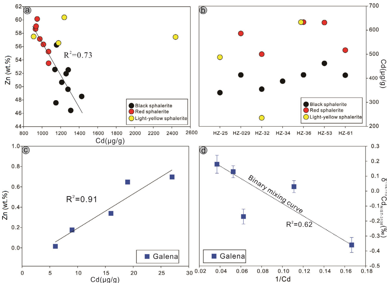
Fig. 5. Plots of (a) Cd–Zn in sphalerite, (b) Cd isotopic compositions of different-colored sphalerite, (c) Cd–Zn in galena, and (d) \delta^{114/110}\text{Cd}-(1/\text{Cd}) for galena.
