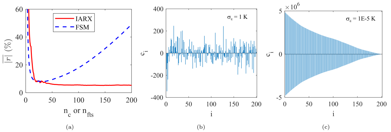
Figure 14: a) Mean residue as a function of the number of future exogenous parameters with IARX ( n_c ) or future time step with FSM ( n_{fts} ); b) IARX future exogenous parameters with n_c = 200 for the tested case with \sigma_\epsilon = 1 \text{ K} ; c) IARX future exogenous parameters with n_c = 200 for the tested case with \sigma_\epsilon = 1\text{E-}5 \text{ K} .
