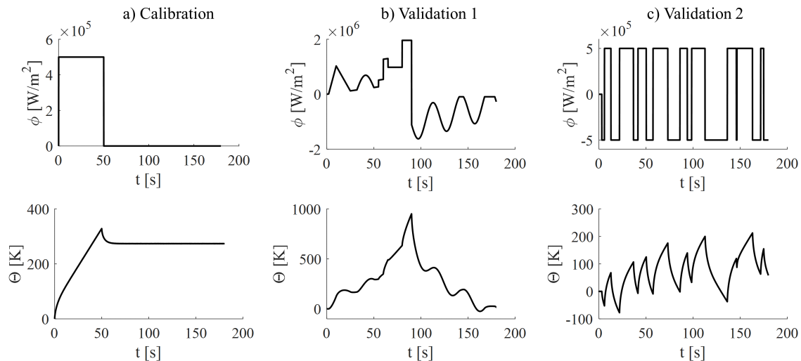
Figure 5: Inputs and outputs used for the calibration and validation steps (reference).
