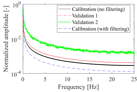
Figure 6: Normalized frequency spectra of the different inputs used in this study (smoothed using 20 neighboring points).
