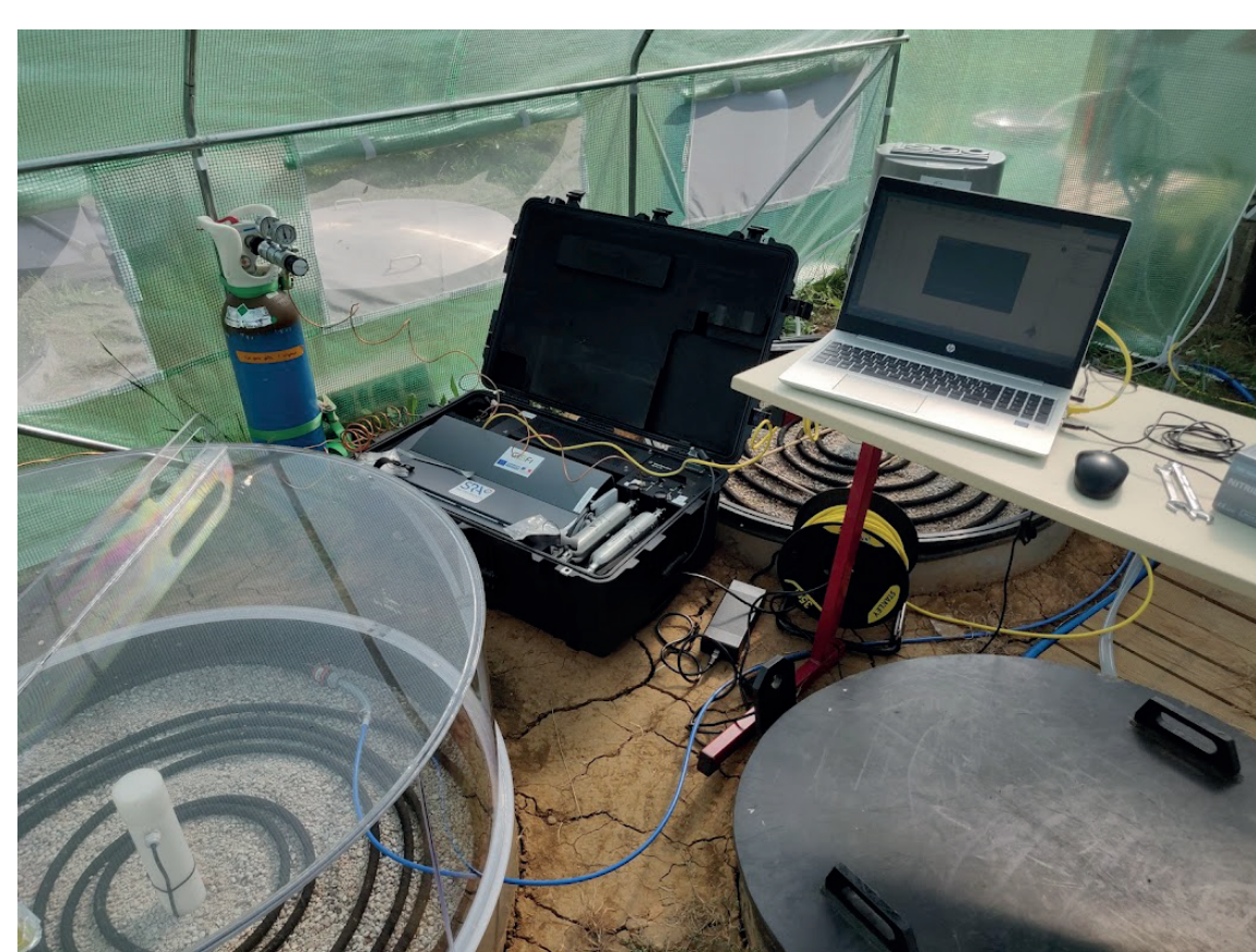
Gas collection chambers and μGC
