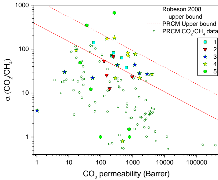
Figure 9. \text{CO}_2/\text{CH}_4 ideal selectivity vs. \text{CO}_2 permeability. PRCM data (from Table 1) and Robeson's 2008 upper bound for polymeric membranes [73]. The dashed line represents the upper bound found for PRCMs in the present review. Featured works: 1 = Okamoto et al. 2001 [121], 2 = Menendez and Fuertes 2001 [139], 3 = Zhou et al. 2001 [140], 4 = Zhou et al. 2003 [128], and 5 = Lee et al. 2016 [157].
