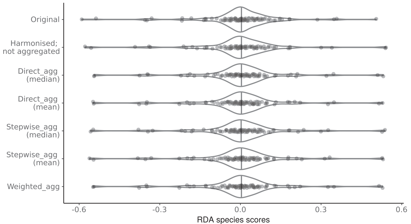
FIGURE 3 Species scores obtained by RDA from the original analysis (Szöcs et al., 2014), using harmonised grouping features, and using harmonised grouping features with traits aggregated to family level with five different aggregation methods. The dots represent the individual species scores for each analysed trait along the conductivity axis. The violin plot shows the density estimate of the species scores. Grey vertical lines indicate the median of the obtained species scores
