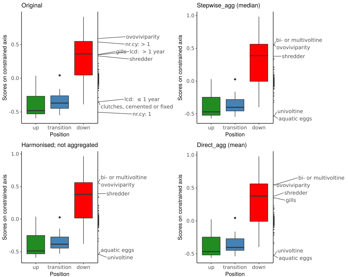
FIGURE 4 RDA of traits constrained by electric conductivity for harmonised but not aggregated data, data aggregated with stepwise_agg median (largest difference in terms of responsive traits to salinity to the original study), data aggregated with direct_agg mean (smallest difference in terms of responsive traits to salinity to the original study), and the original study. Boxplots are shown of the site scores along the conductivity axis. The rug on the right side of each plot indicates species scores of the traits on the conductivity axis. Only traits with a Mahalanobis distance >97.5\% quantile of the \chi^2 distribution (5.02) were labelled. For better comparability, species scores of the original analysis were multiplied by -1 . Results for the other aggregated methods are shown in Figure S7. lcd, life-cycle duration; nr.cy, potential number of cycles per year
