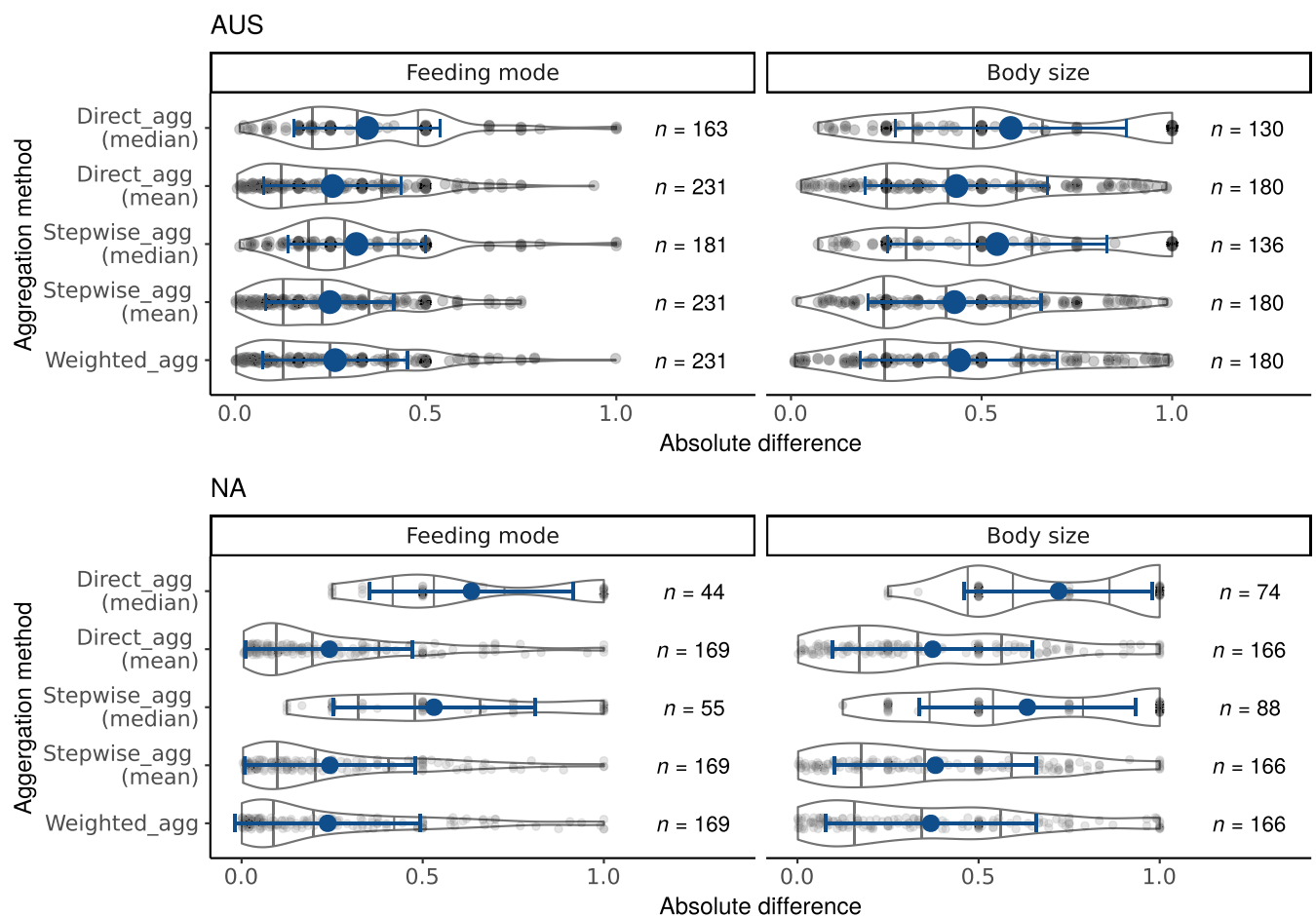
FIGURE 2 Cases (factor combination of investigated families and traits) where differences occurred between aggregated traits and expert assigned traits at the family level for the Australian and North American datasets. Violin plots -- mirrored density plots -- show the density of the absolute trait affinity differences for the grouping features feeding mode and body size. Results for the North American dataset for the grouping features locomotion, respiration, and voltinism are shown in Figure S1. Absolute differences in trait affinities are depicted as grey dots. n denotes the number of cases per comparison where differences occurred. The blue dot indicates the mean of absolute differences, and the error bars show the SD. The grey vertical lines show the 25th, 50th and 75th quantiles of the density estimate. AUS, Australia; NA, North America
