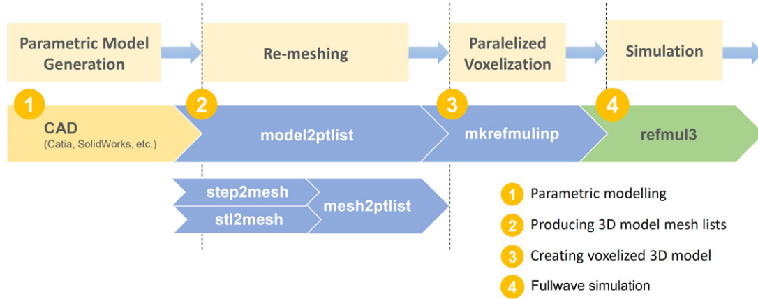
Figure 1. Microwave propagation simulation flow: (1) generation of parameterized real-world models, (2) re-meshing of standardized CAD model output and node and tetrahedron generation, (3) voxelized model generation, (4) fullwave simulation.
