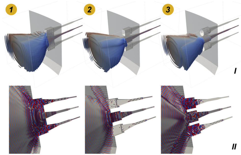
Figure 5. Beam propagation in vacuum, of a 3-antenna cluster, for different 10 cm recessed hole geometries: (1) single common rectangular hole, (2) individual rectangular holes, and (3) individual cylindrical holes.
