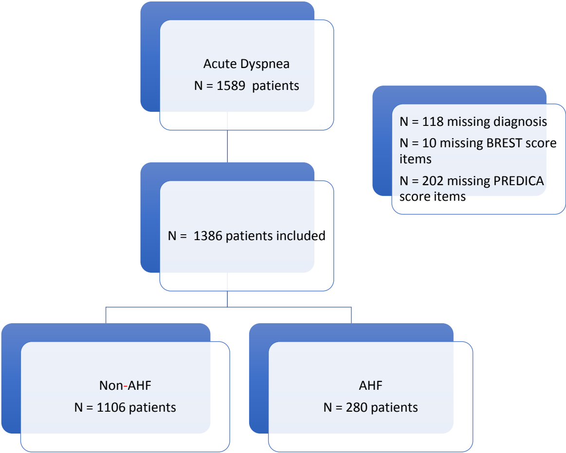
Figure 1. Study flowchart
