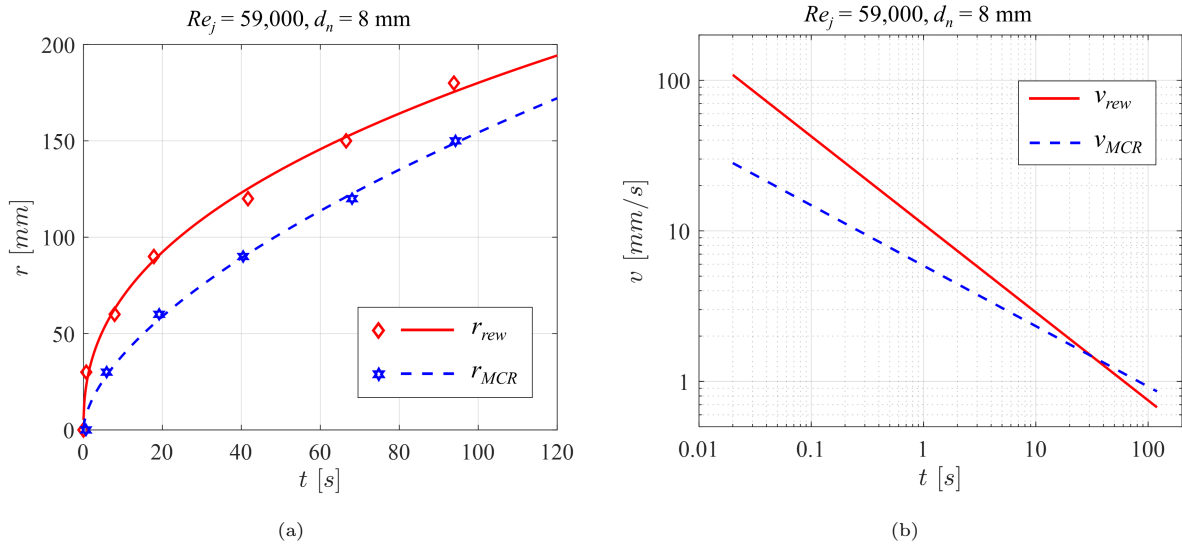
Figure 11: Rewetting characteristics for test 5: a) rewetting and MCR positions, where symbols are the points identified by data processing and lines are fitted power laws; b) rewetting and MCR front velocities estimated with the identified power law coefficients.
