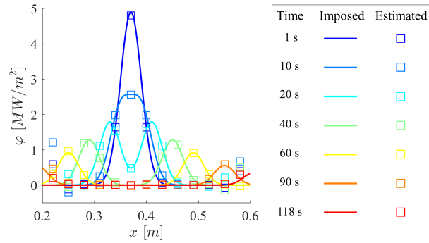
Figure A.20: Comparison between the imposed and estimated heat flux profiles at different times. The symbol's locations correspond to the thermocouples positions in the heated plate.
