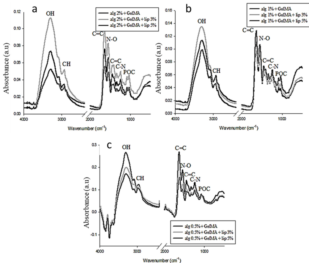
Figure 2. Surface analysis by FTIR of the mixture of GelMA and alginate with different concentrations of alginate. (a) Spectra of the mixtures with 2% ( m/v ) alginate, (b) spectra of the mixtures with 1% ( m/v ) alginate, and (c) spectra of the mixtures with 0.5% ( m/v ) alginate.
