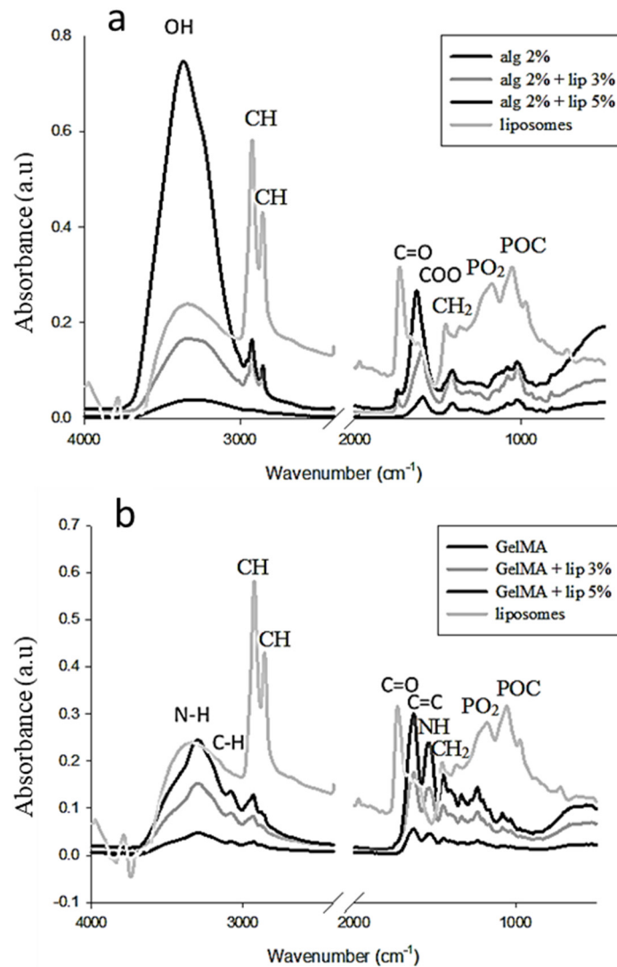
Figure 1. Surface analysis by FTIR of (a) alginate and (b) GelMA before and after functionalization with liposomes (3% and 5% ( w/v )).
