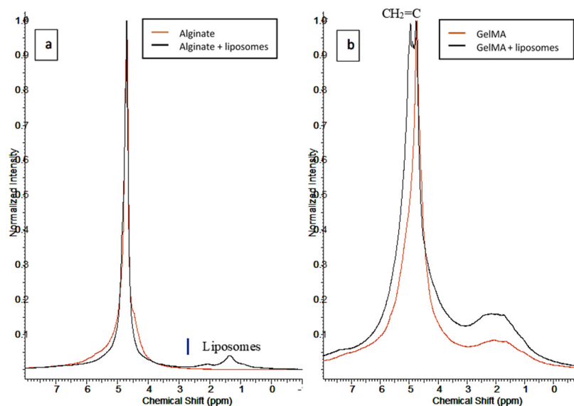
Figure 3. 1 H NMR spectra of (a) alginate and (b) GelMA before and after nanofunctionalization.
