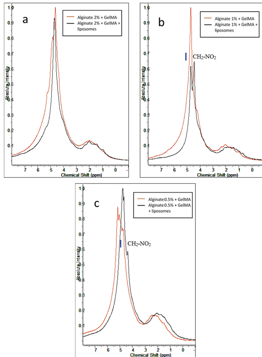
Figure 4. ^1\text{H} NMR spectra of the mixture between GelMA and alginate at different concentrations of alginate with and without nanoliposomes: (a) mixture with 2% alginate, (b) mixture with 1% alginate, and (c) mixture with 0.5% alginate.
