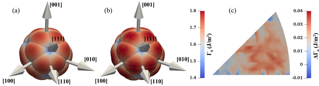
Figure 6: 3D surface plots of \Gamma_0 for Ni free surfaces calculated by (a) Herring’s method without atomic relaxation [54] and (b) semi-analytical method considering atomic relaxation, (c) IPF representation of the difference of \Gamma_0 between (b) and (a) presented in the IPF.
