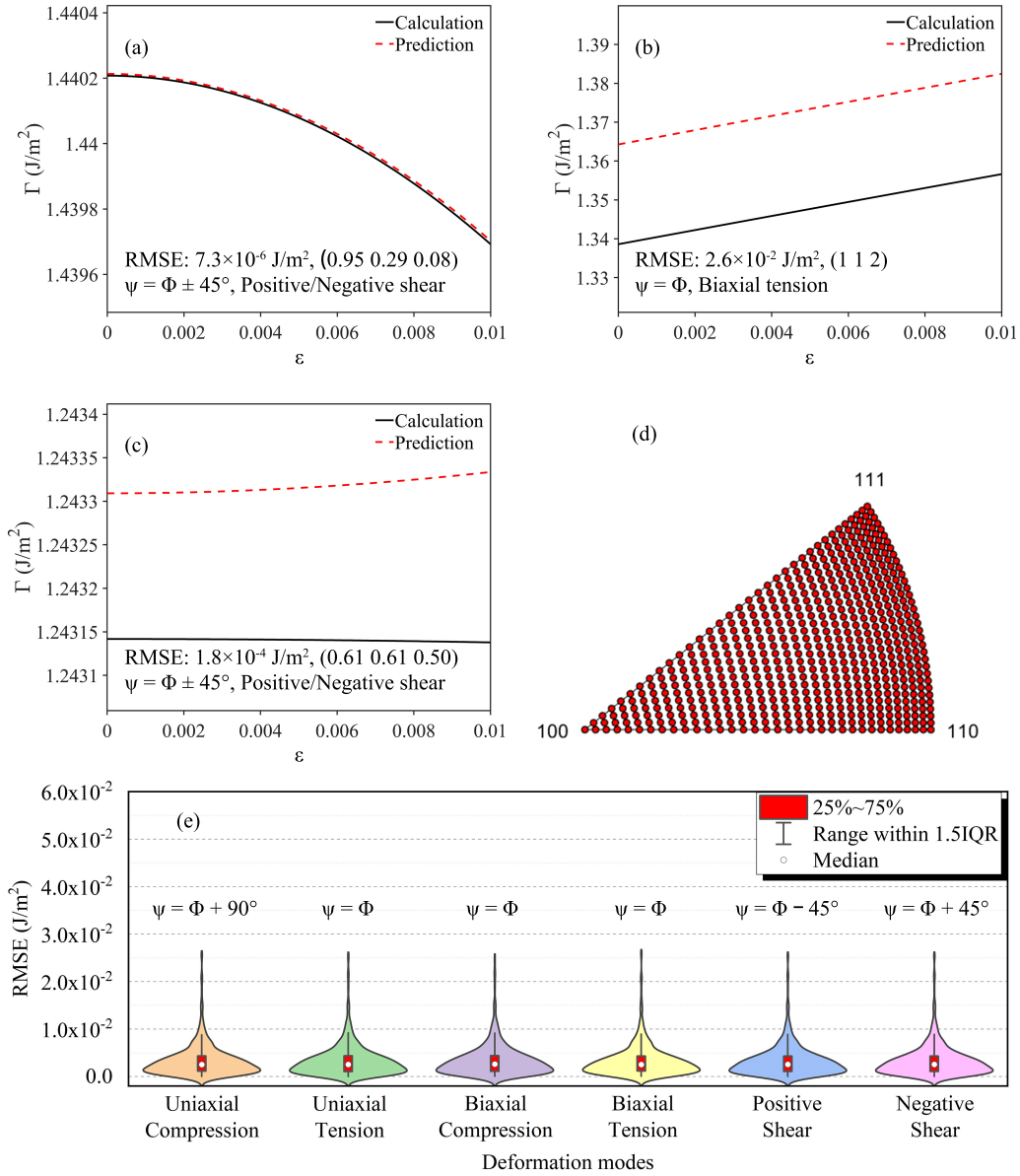
Figure 16: Comparison between the predicted evolution of \Gamma and the calculated one (see Eqs. (3) and (14)) with : (a) the best RMSE score, (b) the worst RMSE score and (c) the inverse tendency, among 595 verified Cu surfaces (see Fig. (d)) and 6 deformation modes. (d) 595 uniform surface orientations presented in the IPF. (e) The distribution of RMSE scores of 595 verified Cu surfaces (see Fig. (d)) and 6 deformation modes with \epsilon \in [0, 0.01] .
