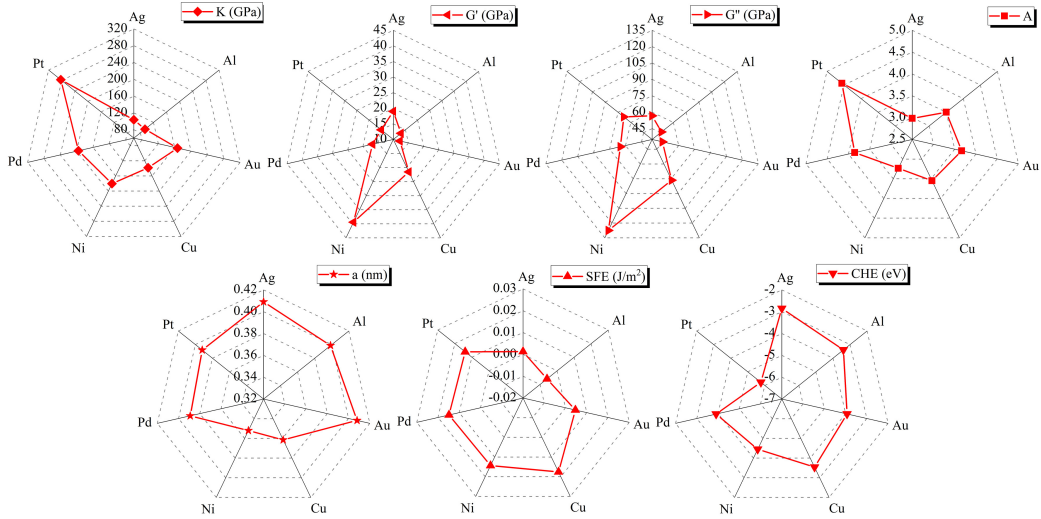
Figure 5: Material’s bulk parameters: K (the bulk modulus, in GPa), G' (the \{001\} \langle 110 \rangle shear resistance, in GPa), G'' (the \{001\} \langle 100 \rangle shear resistance, in GPa), A (the elastic anisotropy ratio), a (the lattice parameter, in nm), SFE (the stacking fault energy, in \text{J}/\text{m}^2 ) and CHE (the cohesive energy, in eV) used in BRT models for all the studied materials.
