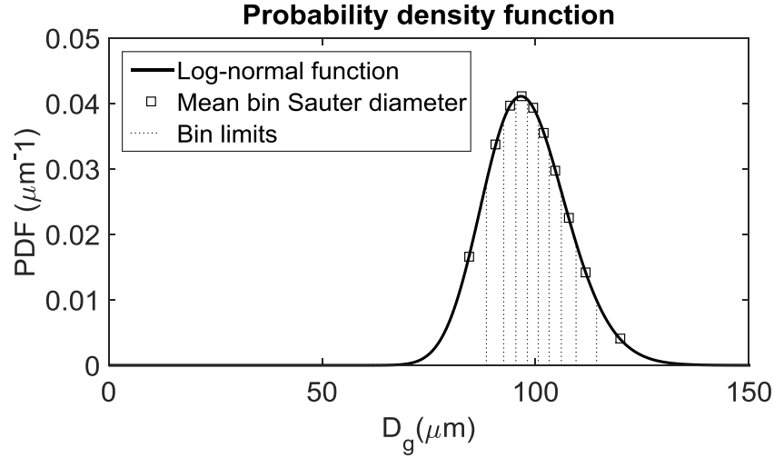
Figure 3. Log-normal distribution for \sigma=0.10 and d_{oo}=100 \mu\text{m} . 10 bins
