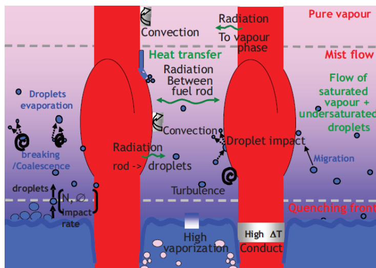
Fig. 2. Thermal-hydraulic phenomena occurring during the reflooding phase of a LOCA at the sub-channel scale [4]
