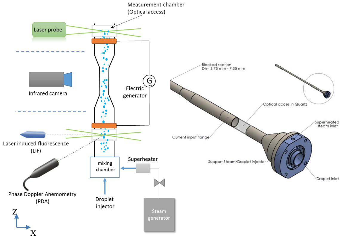
Fig. 5. Scheme of thermal hydraulic circuit of the experimental test facility
