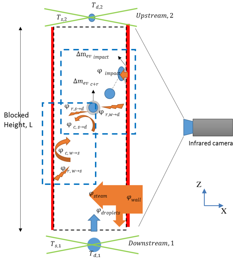
Fig. 9. Scheme of the different heat exchanges along the blocked area of the Venturi tube. (D:Droplet, S:Steam, W:Wall, C:Convection, R:Radiation)
