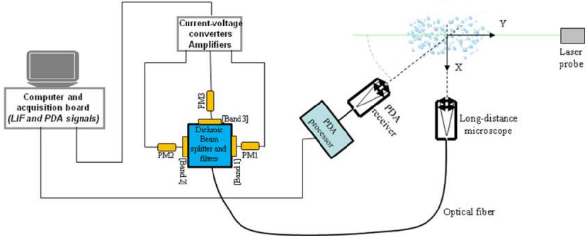
Fig. 8. LIF/PDA optical setup [19]
