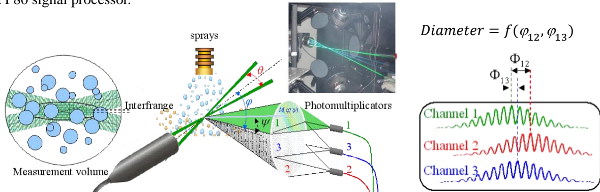
Fig. 6. PDA technics
