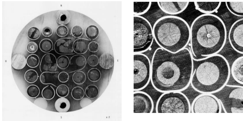
Fig. 1. Bundle of deformed fuel rods; Phebus LOCA experiments (1983)
