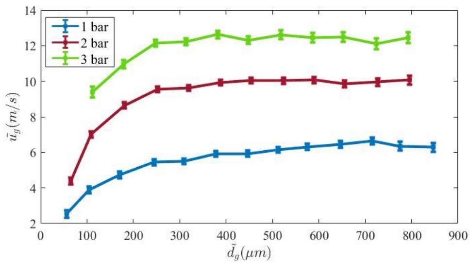
Figure 5. Velocity/Diameter correlation with three pressure levels and a fixed duty cycle of 50%
