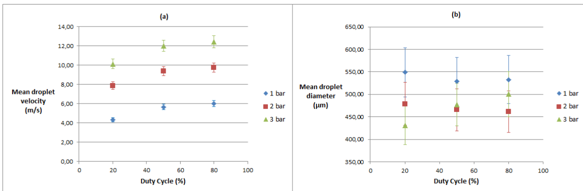
Figure 6. Droplet characteristics mean values for all PDA experiments.
