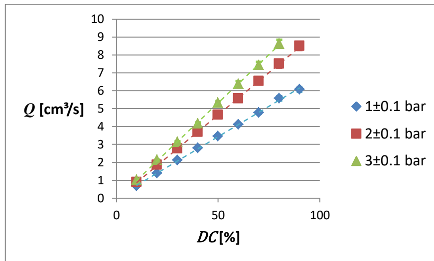
Figure 2. Measurements points for mass flow rate according to pressure and duty cycle
