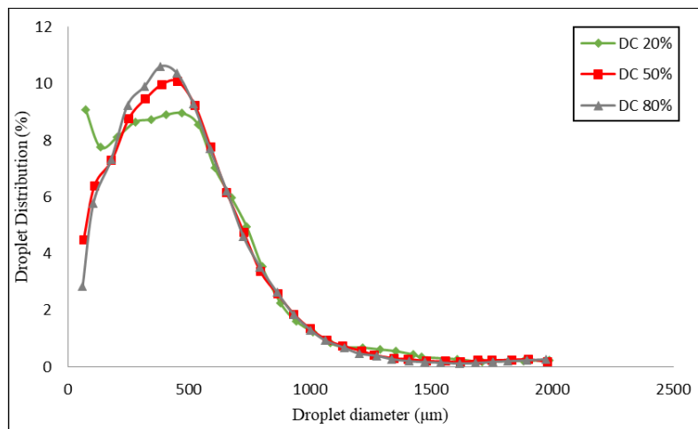
Figure 8. Droplet diameter distribution for three values of duty cycle and fixed pressure of 2 bar.
