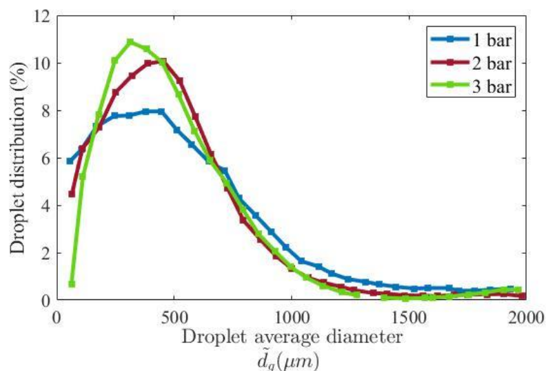
Figure 3. Distribution of the droplets average diameter for three levels of pressure with a duty cycle of 50%
