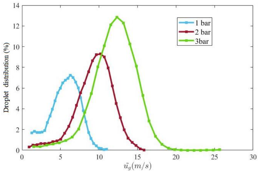
Figure 4. Distribution of the droplet's average velocity for three levels of pressure with a duty cycle of 50%
