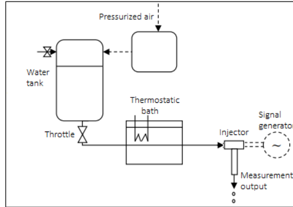
Figure 1. Simplified scheme of experimental procedure
