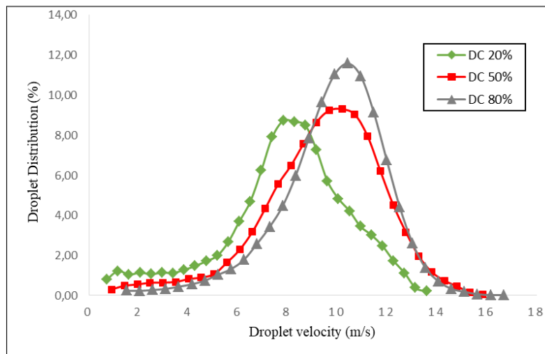
Figure 7. Droplet velocity distribution for three values of duty cycle and fixed pressure of 2 bar.
