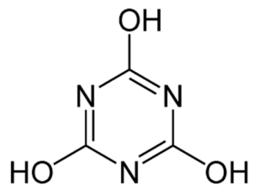
Figure 3. Cyanuric acid (HNCO) 3 - 1,3,5-triazine-2,4,6-triol.
