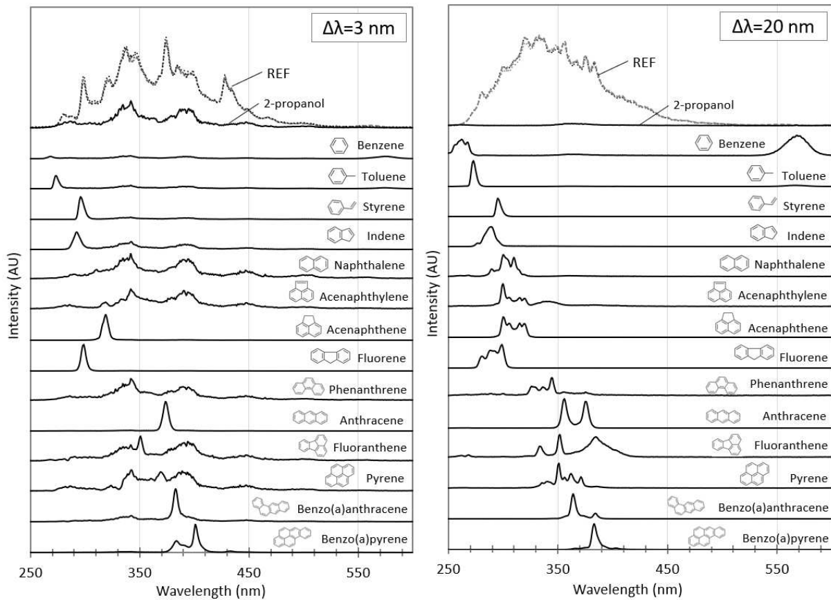
374 375 Figure 4: Synchronous Fluorescence spectra recorded at offset=3 nm (left) and offset=20 nm (right) of three reference 376 experiments, 2-propanol and 14 model molecules.
