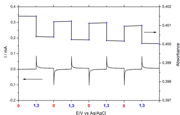
Figure 4. Variation of the absorbance of [\text{Fe}(\text{bpy})_2(\text{bpy}')]^{2+} -functionalized films at a probe wavelength of 525 nm upon double step chronoamperometry between 0 and +1.3V (pulse width: 10 s).
