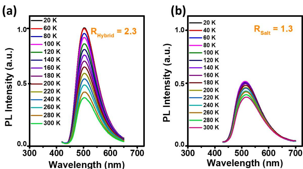
Fig. 4 (a-b) Temperature dependence PL of [HQ] 2 SnCl 6 ·2H 2 O and the (HQ.Cl) salt respectively measured under 375 nm excitation.
