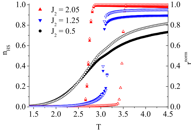
FIG. 1: (color online) HS fraction n_{HS} (open symb.) and normalized lattice spacing r^{norm} (filled symb.) as a function of temperature, for different values of the J_2 coupling parameter. Thermal cycles have been computed as in ref. 47 , using the Metropolis MC dynamic for the two variables, thermal averages have been computed over 5000 independant MC simulations. Model parameters: J_0 = 1000 , J_1 = 0.15 , \Delta = 7.2 and \ln g = 2 .
