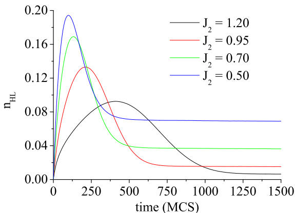
FIG. 9: (color online) Temporal evolution of the fraction of HS-LS pairs n_{HL} for different "weak" values of the J_2 parameter.
