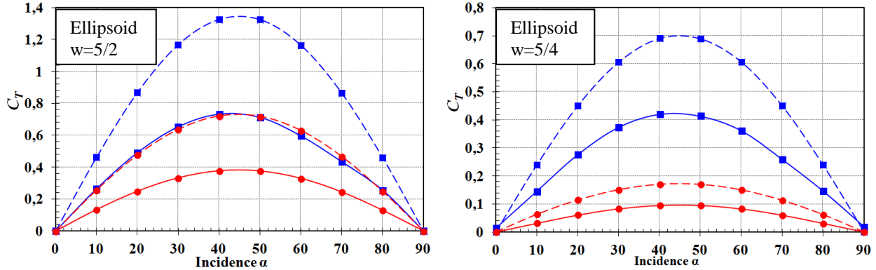
Figure 6. Comparison of the torque coefficients for different particles Reynolds numbers. Present results: (■); results of Zastawny et al. [8]: (●). The dashed lines are referred to Re_p = 10 and the continuous lines are referred to Re_p = 300 .
