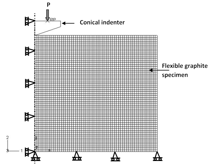
Figure 4. FE model and boundary conditions
