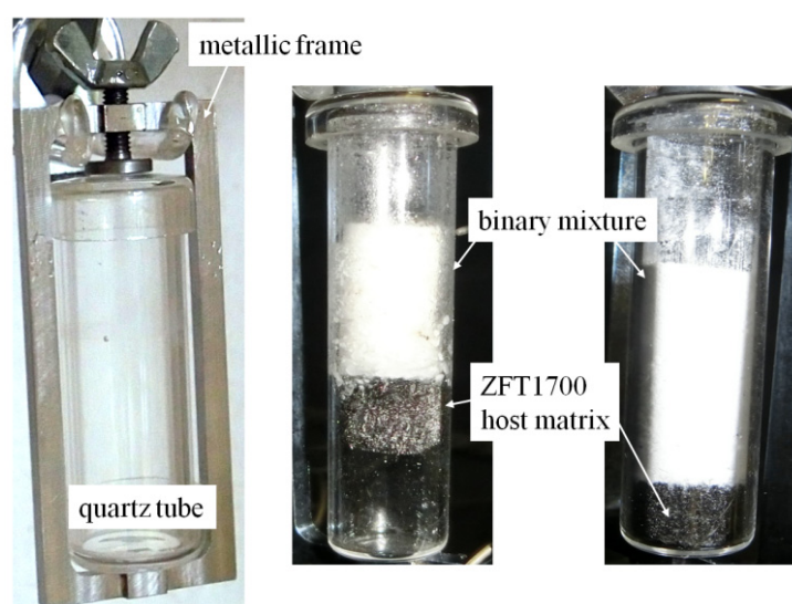
Fig. 2 Infiltration device with the host matrix placed in the middle and at the bottom of the quartz tube.
