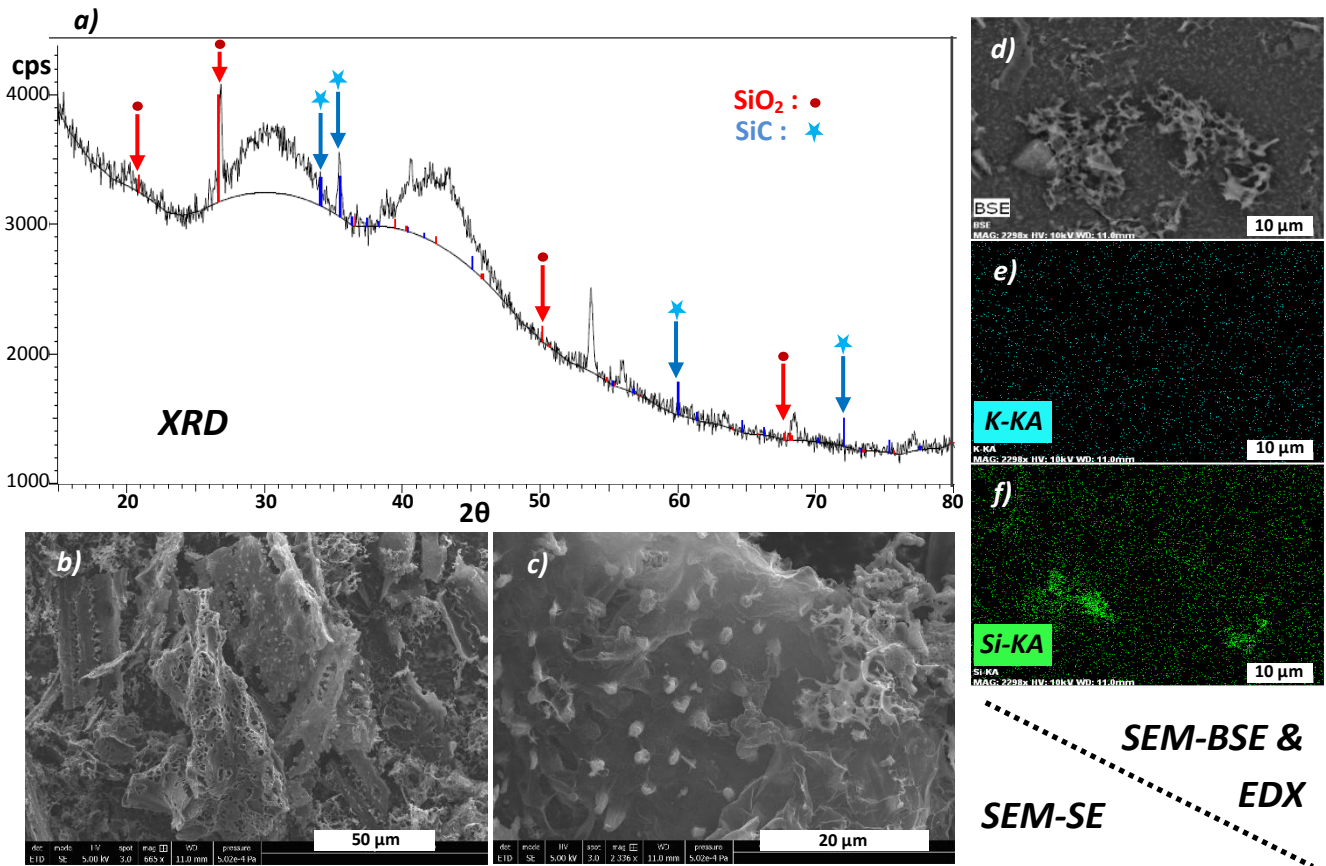
Figure 1: (a) XRD pattern and assignation of the \text{SiO}_2 and \text{SiC} peaks for KC-RS_3 sample, (b) and (c) SEM-SE pictures of KC-RS_3, (d) SEM-BSE picture of KC-RS_3, (e) and (f) EDX mapping of (d) for K and Si, respectively.
